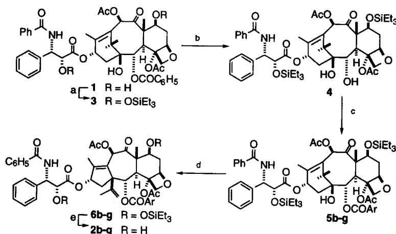
Scheme 1. (a) Et 3 SiCl, imidazole, DMF, rt, 1 h, 3 , 95%. (b) Bu 3 NHSO 4 , 2 N NaOH, C 6 H 6 , CH 2 Cl 2 , rt, 1 h, 4 , 65%. (c) ArCOOH, DCC, 4-PP, C 6 H 5 CH 3 , 5b-g , 65–75%. (d) SOCl 2 , py, CH 2 Cl 2 , rt, 6b-g , 40–65%. (e) MeOH/5%/HCl, rt, 2b-g , 90–95%.
